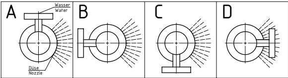
Figure 4: Water Connection Flange Options
